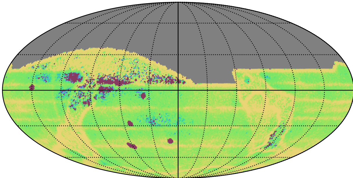
ddf_acor_sf20_lsf0_lsr0_v3.4_10yrs All sky: Median Intra-Night Gap
