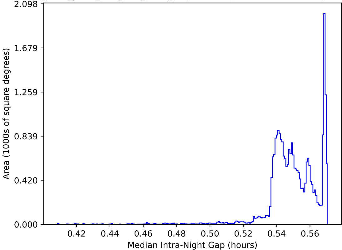
ddf_acor_sf20_lsf0_lsr0_v3.4_10yrs All sky: Median Intra-Night Gap
