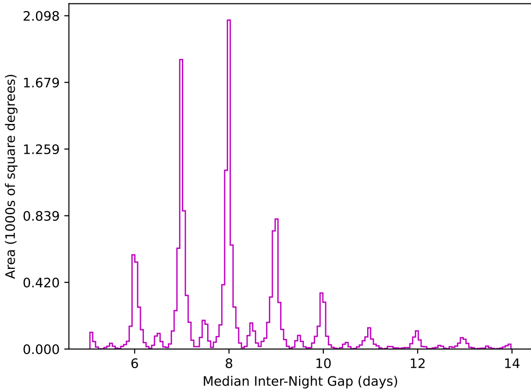
ddf_acor_sf20_lsf0_lsr0_v3.4_10yrs WFD z band: Median Inter-Night Gap
