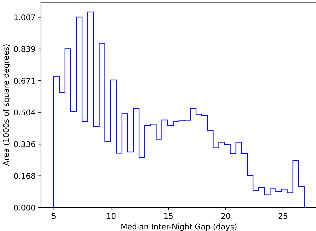
ddf_acor_sf20_lsf0_lsr0_v3.4_10yrs WFD y band: Median Inter-Night Gap
