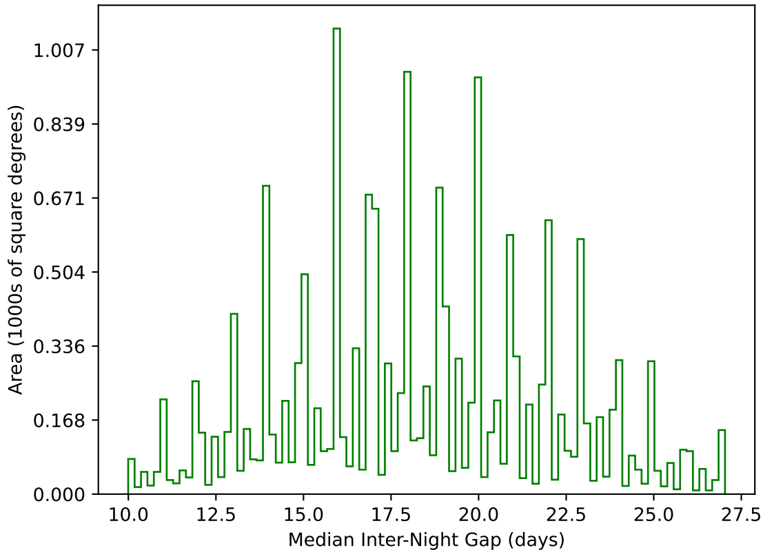
ddf_acor_sf20_lsf0_lsr0_v3.4_10yrs WFD g band: Median Inter-Night Gap
