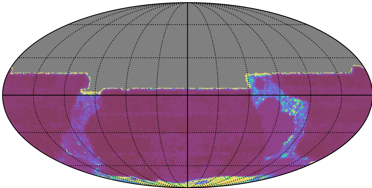
ddf_acor_sf20_lsf0_lsr0_v3.4_10yrs All sky y band: Median Inter-Night Gap
