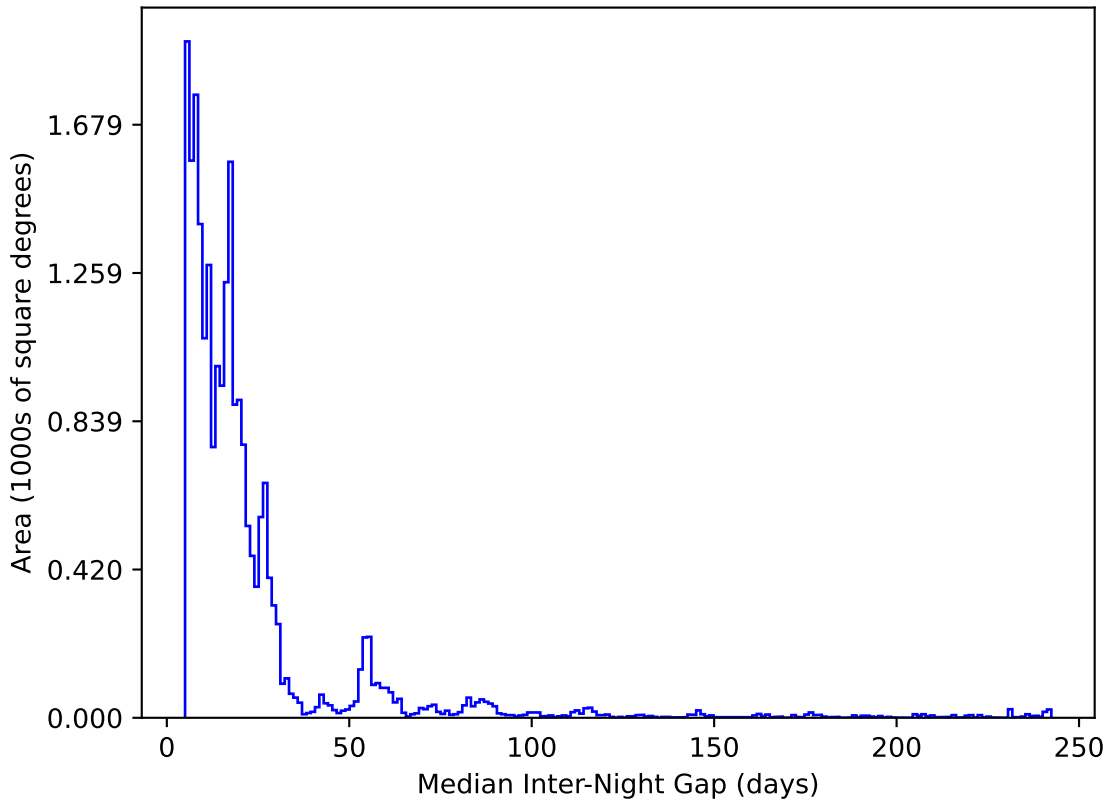
ddf_acor_sf20_lsf0_lsr0_v3.4_10yrs All sky y band: Median Inter-Night Gap
