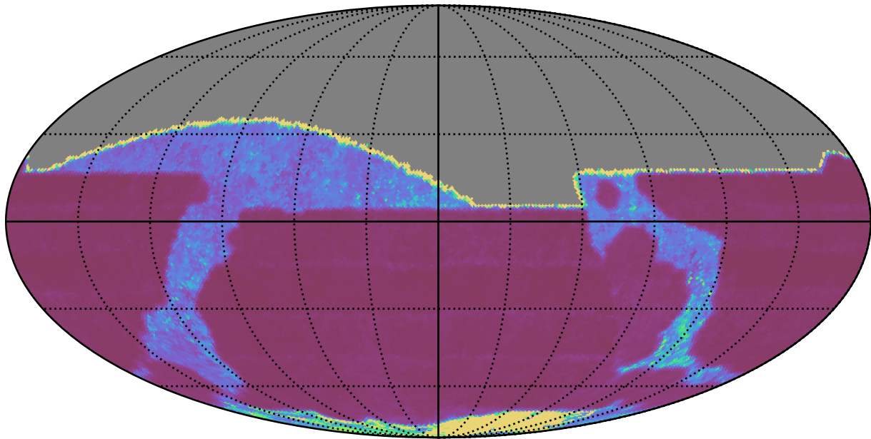
ddf_acor_sf20_lsf0_lsr0_v3.4_10yrs All sky r band: Median Inter-Night Gap
