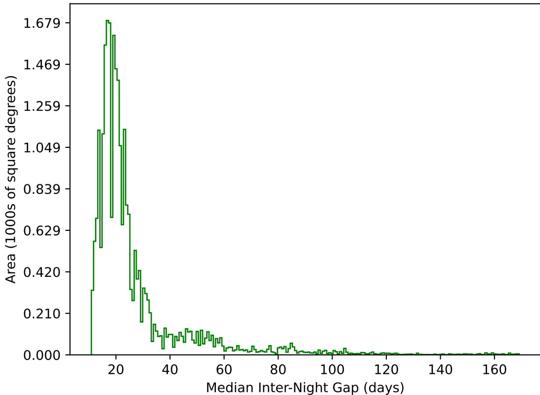
ddf_acor_sf20_lsf0_lsr0_v3.4_10yrs All sky g band: Median Inter-Night Gap
