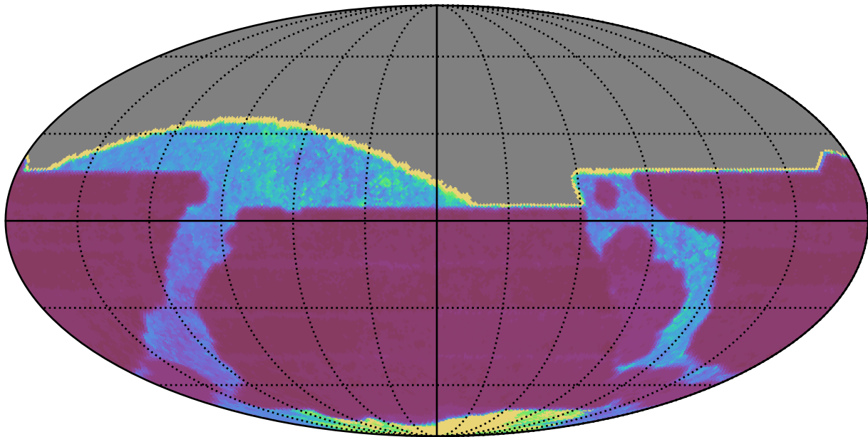
ddf_acor_sf20_lsf0_lsr0_v3.4_10yrs All sky all bands: Median Inter-Night Gap
