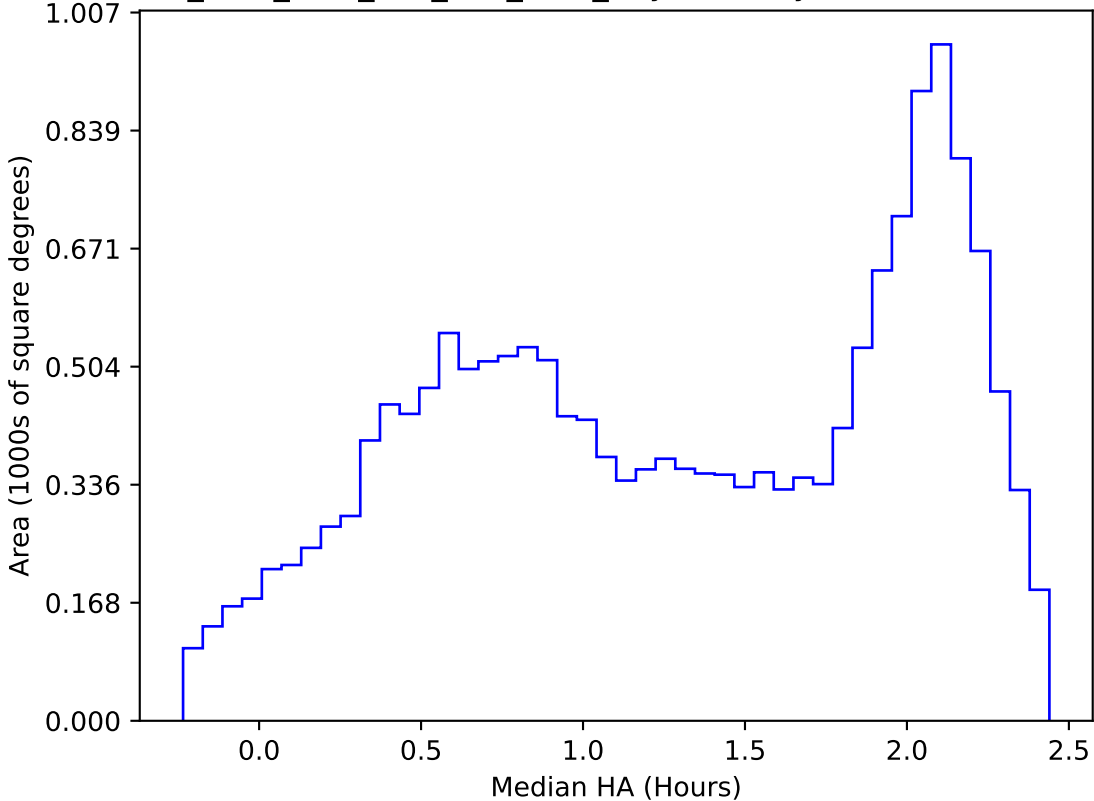
ddf_acor_sf20_ls0_lsr0_v3.4_10yrs WFD y band: Median HA
