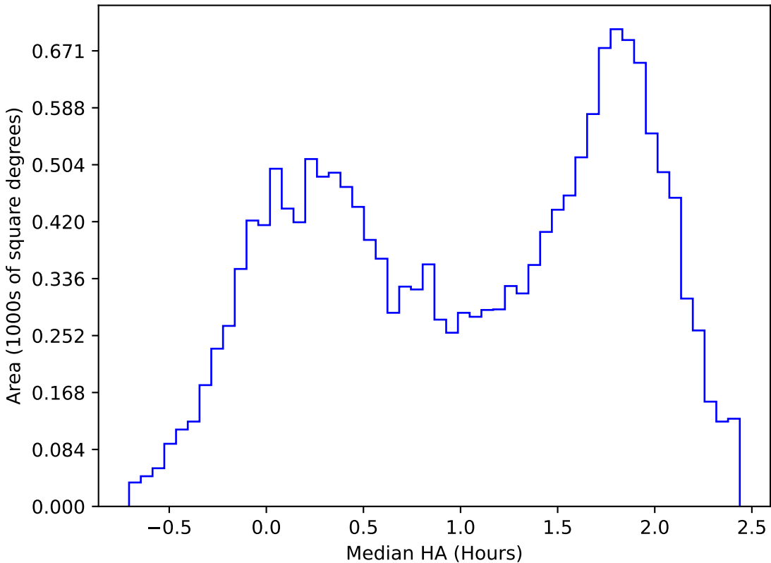
ddf_acor_sf20_lsf0_lsr0_v3.4_10yrs WFD u band: Median HA
