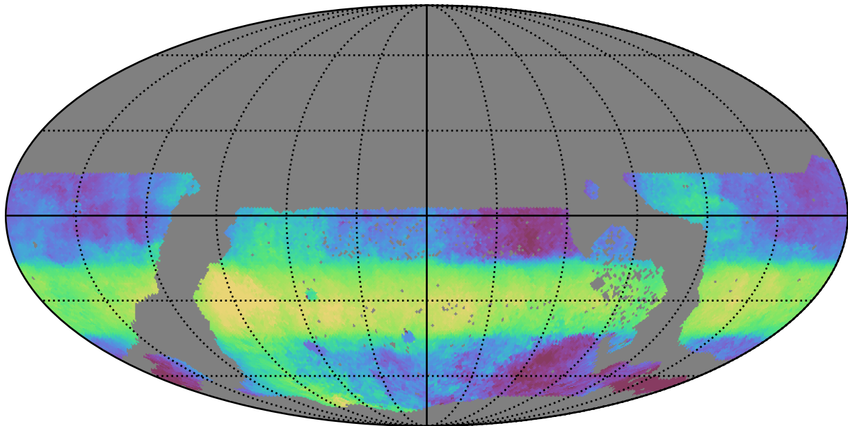
ddf_acor_sf20_lsf0_lsr0_v3.4_10yrs WFD r band: Median HA
