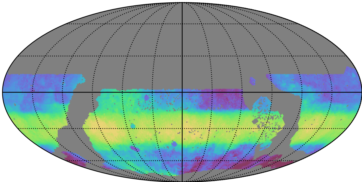
ddf_acor_sf20_lsf0_lsr0_v3.4_10yrs WFD i band: Median HA
