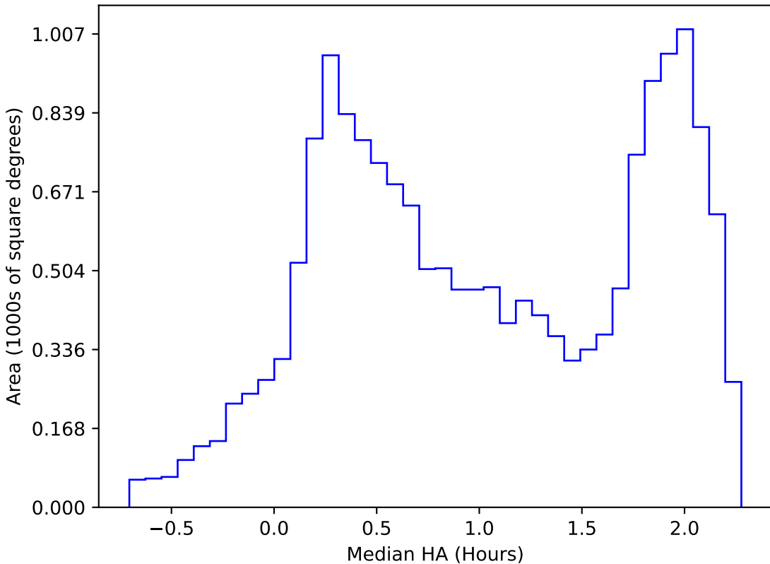
ddf_acor_sf20_lsf0_lsr0_v3.4_10yrs WFD i band: Median HA
