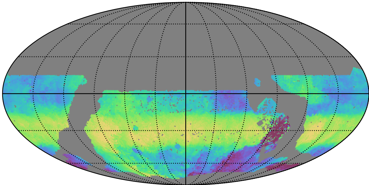
ddf_acor_sf20_lsf0_lsr0_v3.4_10yrs WFD g band: Median HA
