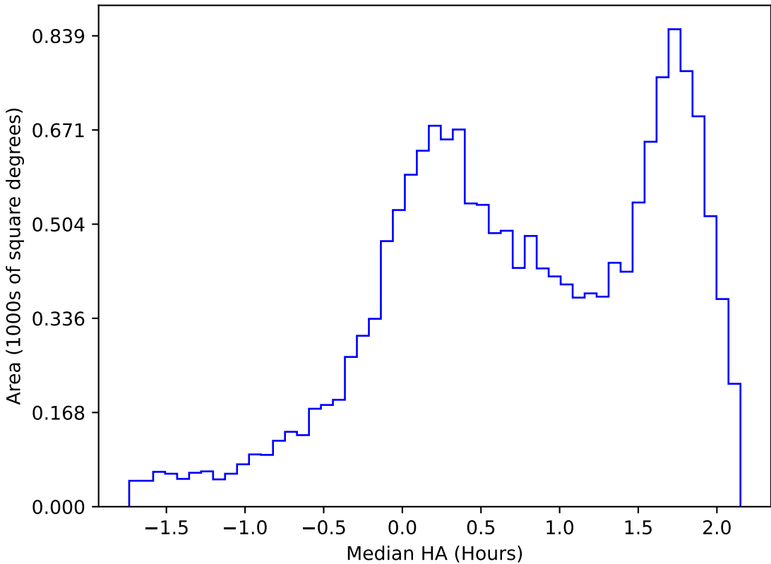
ddf_acor_sf20_ls0_lsr0_v3.4_10yrs WFD g band: Median HA
