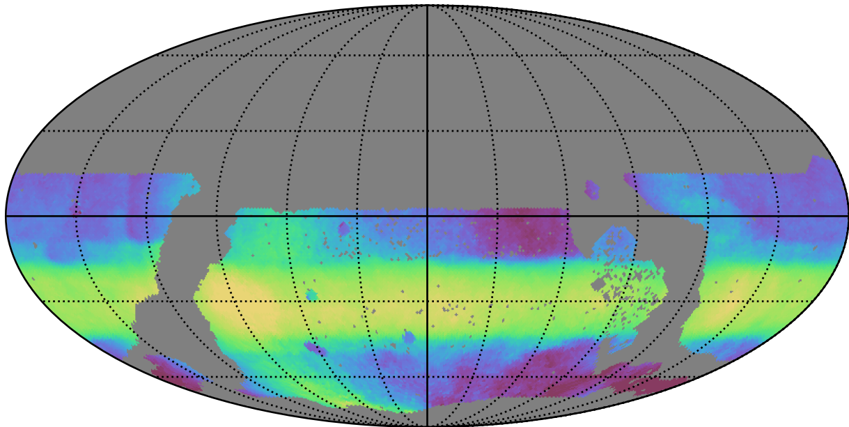
ddf_acor_sf20_lsf0_lsr0_v3.4_10yrs WFD all bands: Median HA
