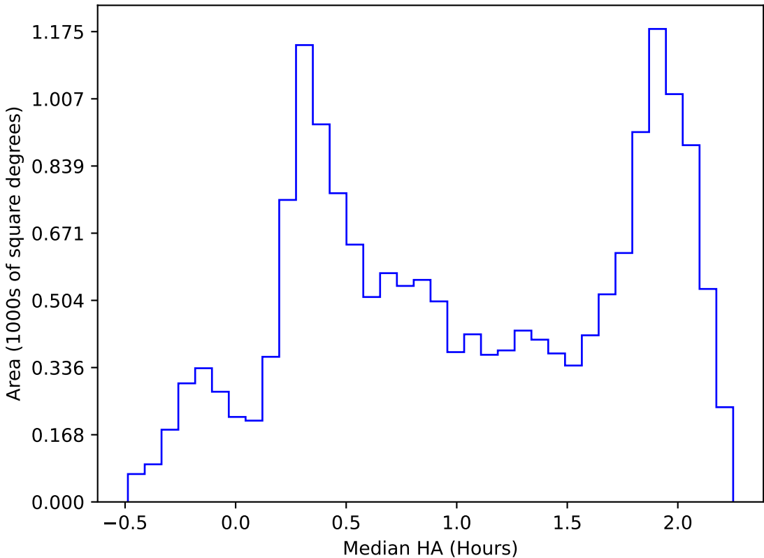
ddf_acor_sf20_lsf0_lsr0_v3.4_10yrs WFD all bands: Median HA
