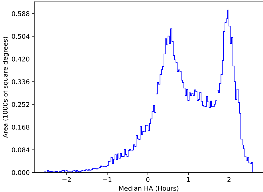
ddf_acor_sf20_lsf0_lsr0_v3.4_10yrs All sky z band: Median HA
