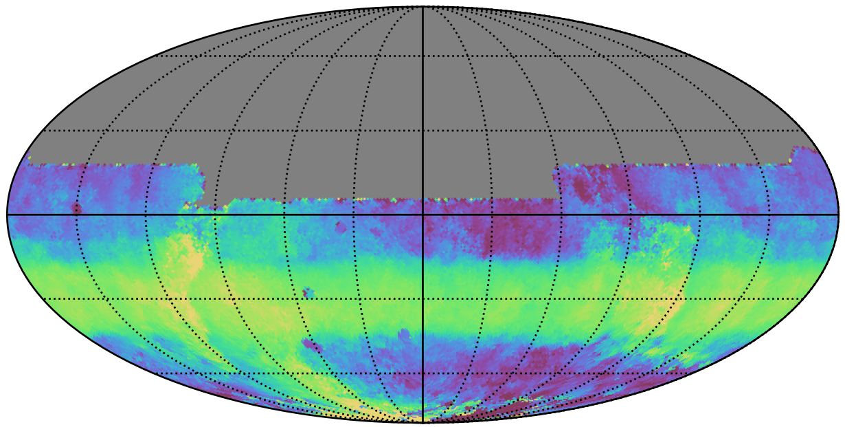
ddf_acor_sf20_lsf0_lsr0_v3.4_10yrs All sky y band: Median HA
