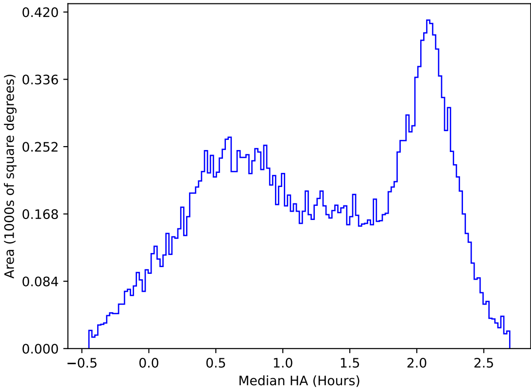
ddf_acor_sf20_lsf0_lsr0_v3.4_10yrs All sky y band: Median HA
