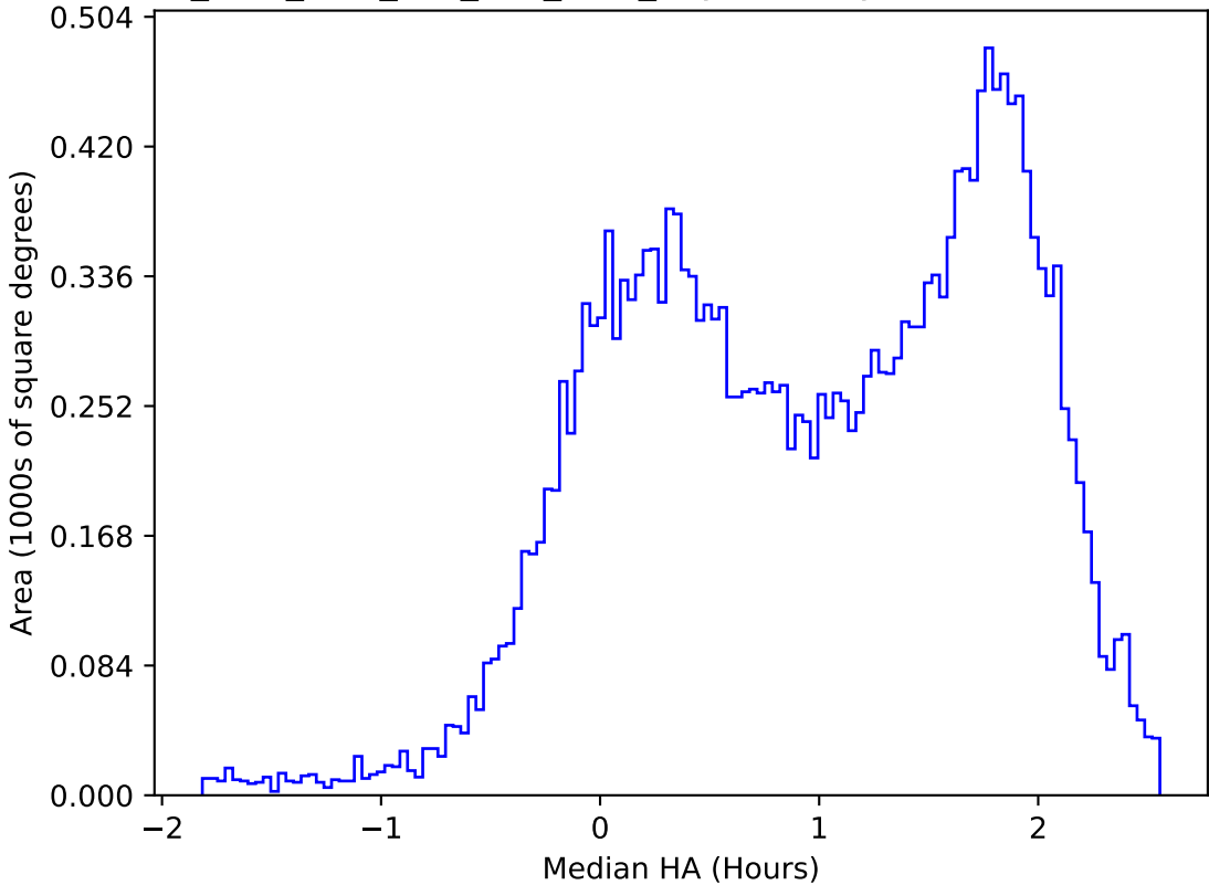
ddf_acor_sf20_lsf0_lsr0_v3.4_10yrs All sky u band: Median HA
