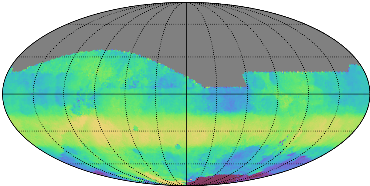
ddf_acor_sf20_lsf0_lsr0_v3.4_10yrs All sky r band: Median HA
