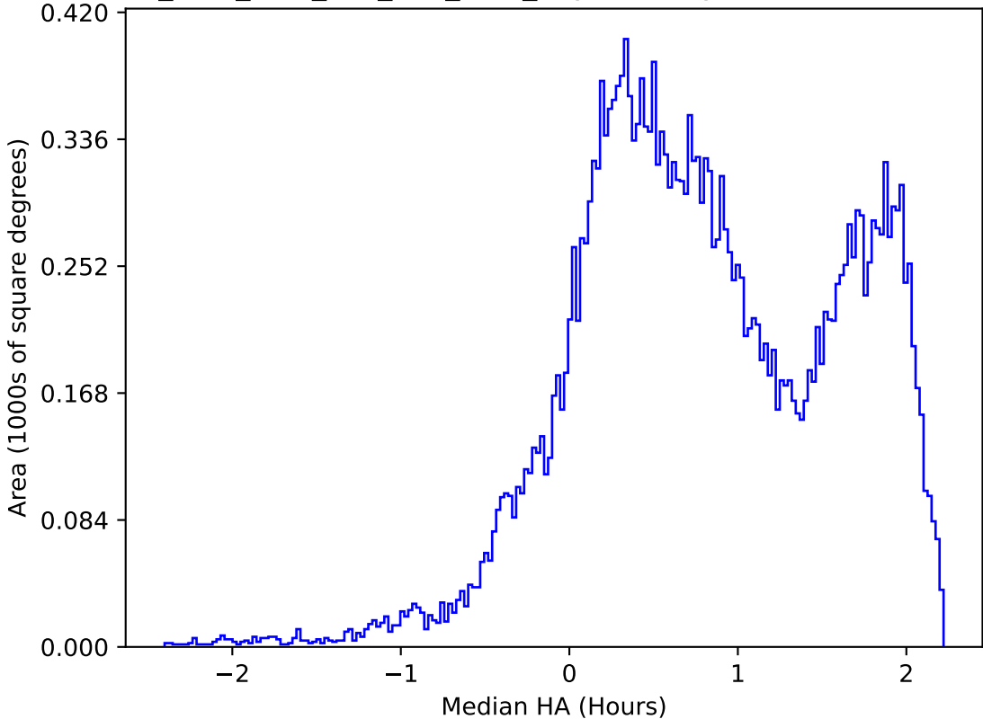
ddf_acor_sf20_lsf0_lsr0_v3.4_10yrs All sky r band: Median HA
