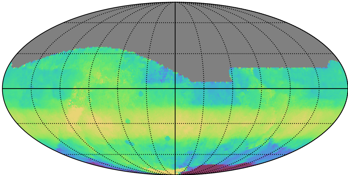
ddf_acor_sf20_lsf0_lsr0_v3.4_10yrs All sky i band: Median HA
