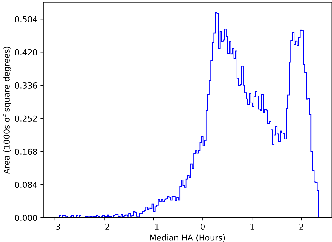
ddf_acor_sf20_lsf0_lsr0_v3.4_10yrs All sky i band: Median HA
