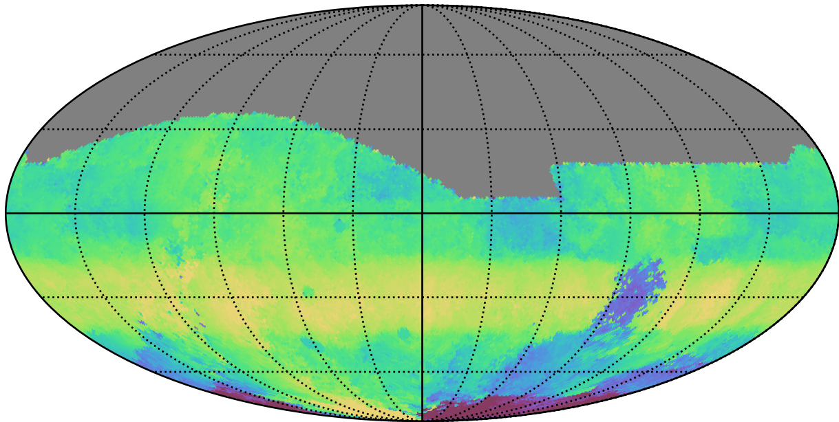
ddf_acor_sf20_lsf0_lsr0_v3.4_10yrs All sky g band: Median HA
