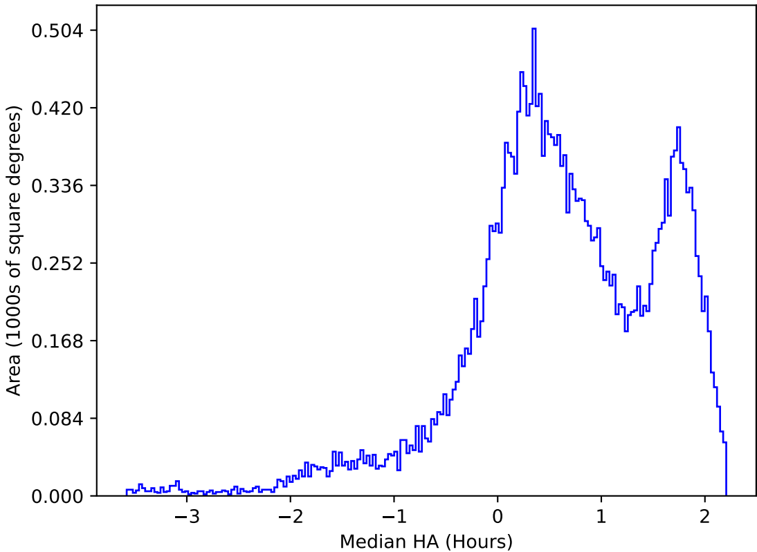
ddf_acor_sf20_lsf0_lsr0_v3.4_10yrs All sky g band: Median HA
