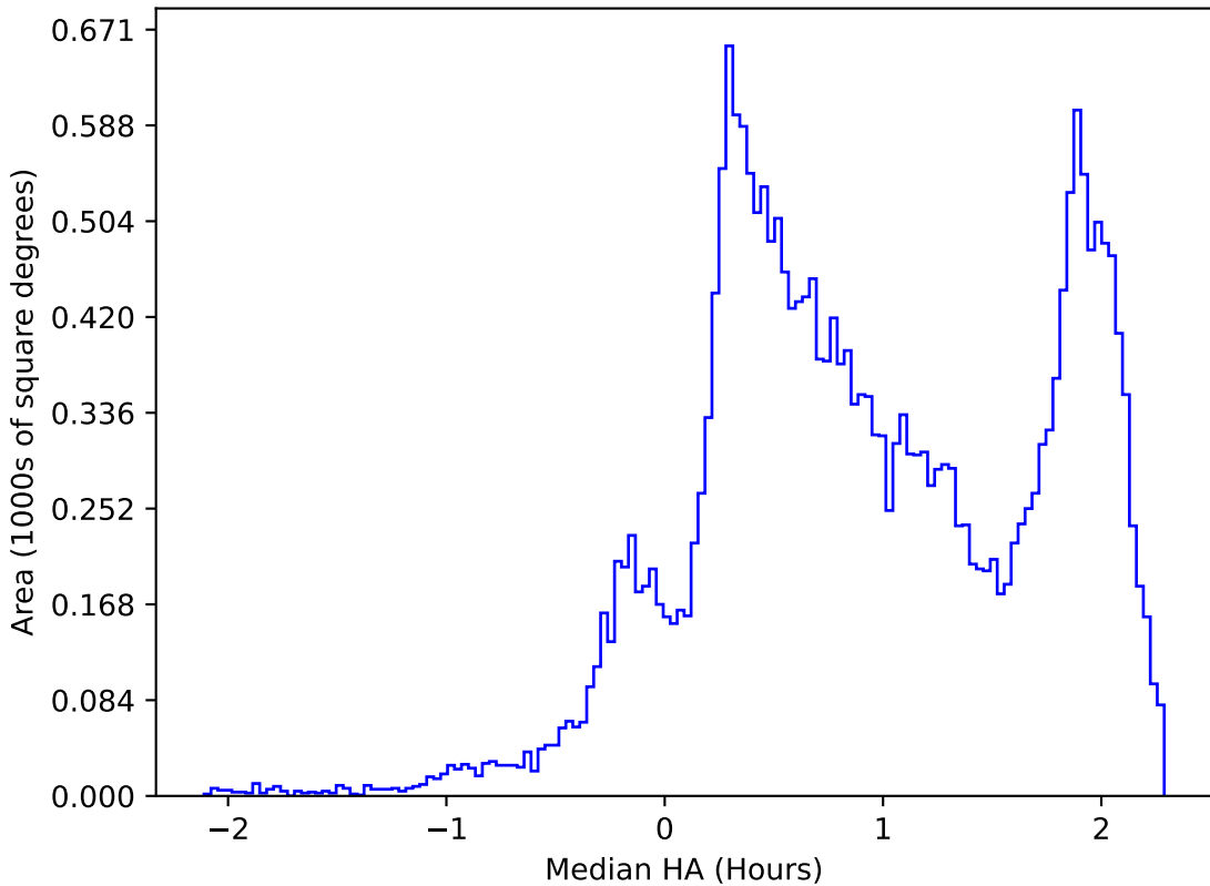
ddf_acor_sf20_lsf0_lsr0_v3.4_10yrs All sky all bands: Median HA
