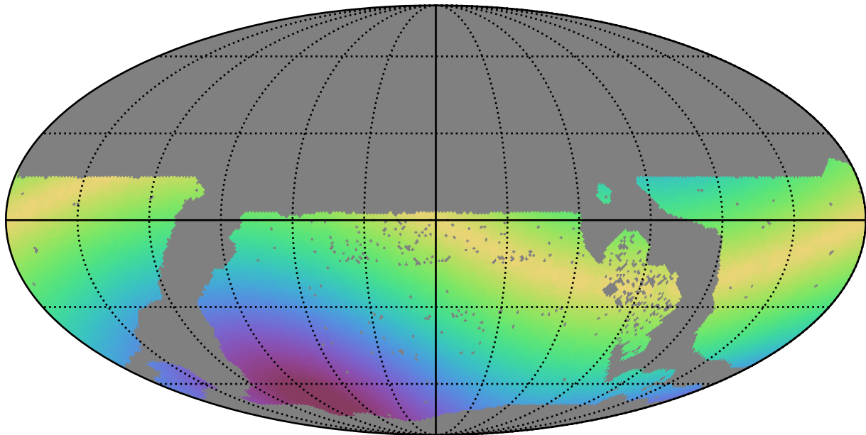
ddf_acor_sf20_lsf0_lsr0_v3.4_10yrs WFD z band: Max solarElong
