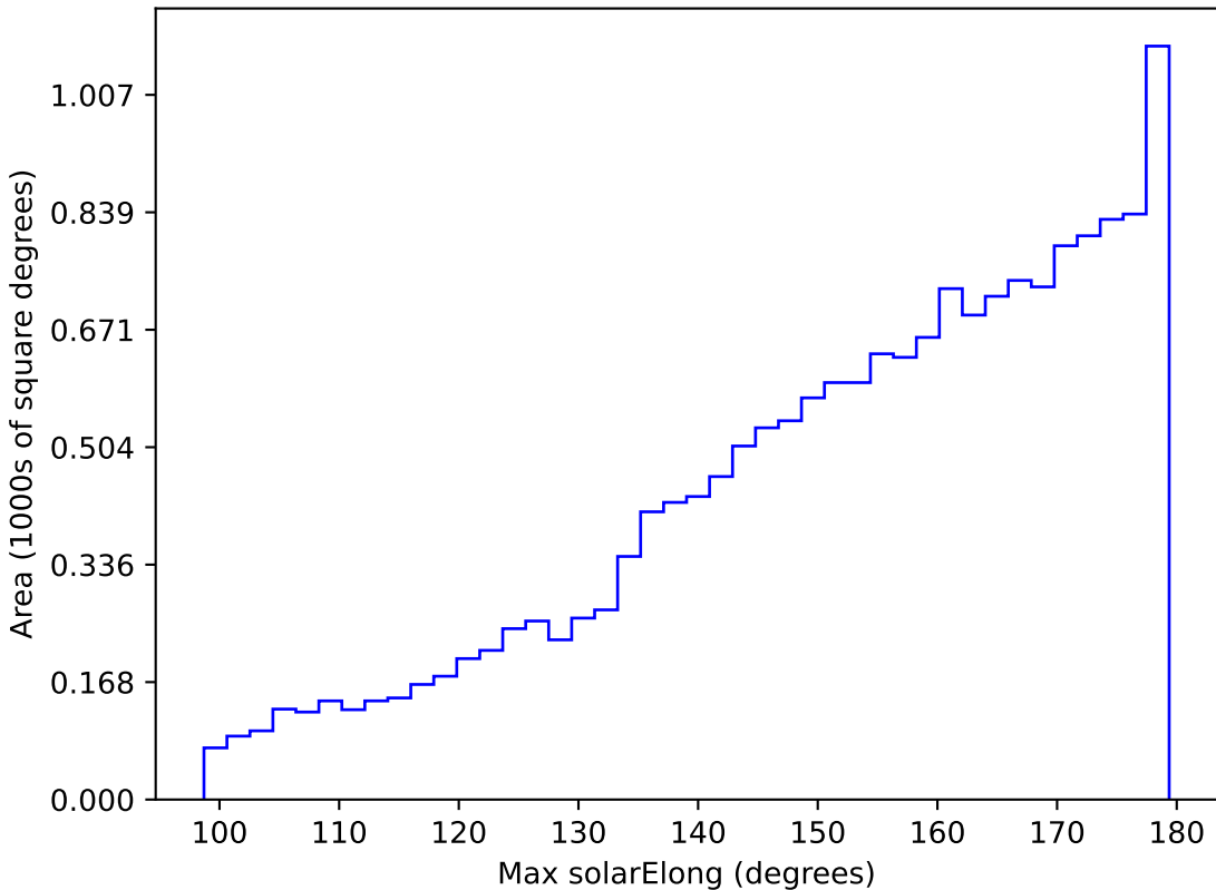
ddf_acor_sf20_lsf0_lsr0_v3.4_10yrs WFD z band: Max solarElong
