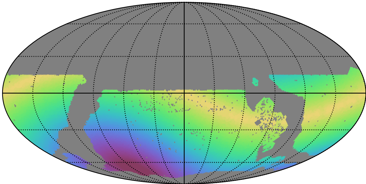
ddf_acor_sf20_lsf0_lsr0_v3.4_10yrs WFD y band: Max solarElong
