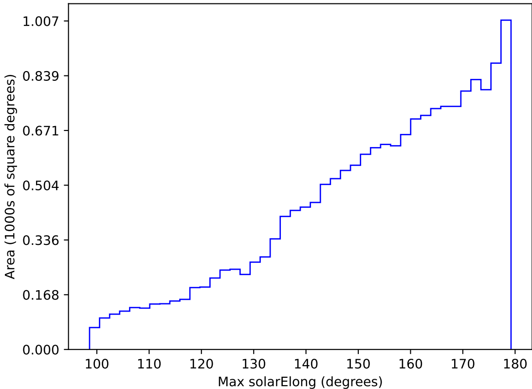
ddf_acor_sf20_lsf0_lsr0_v3.4_10yrs WFD y band: Max solarElong
