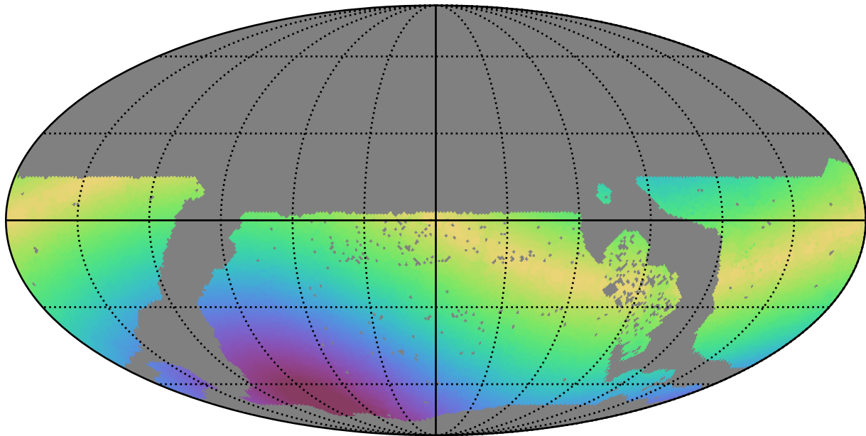
ddf_acor_sf20_lsf0_lsr0_v3.4_10yrs WFD u band: Max solarElong
