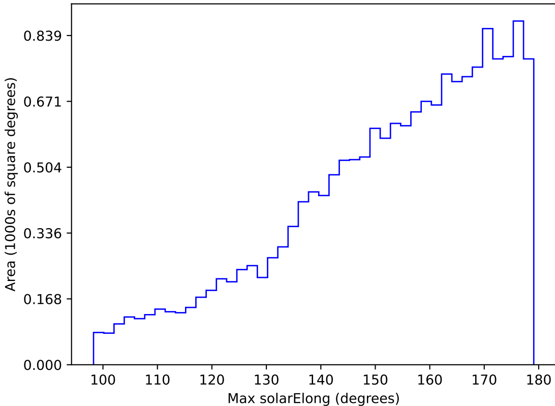
ddf_acor_sf20_ls0_lsr0_v3.4_10yrs WFD u band: Max solarElong
