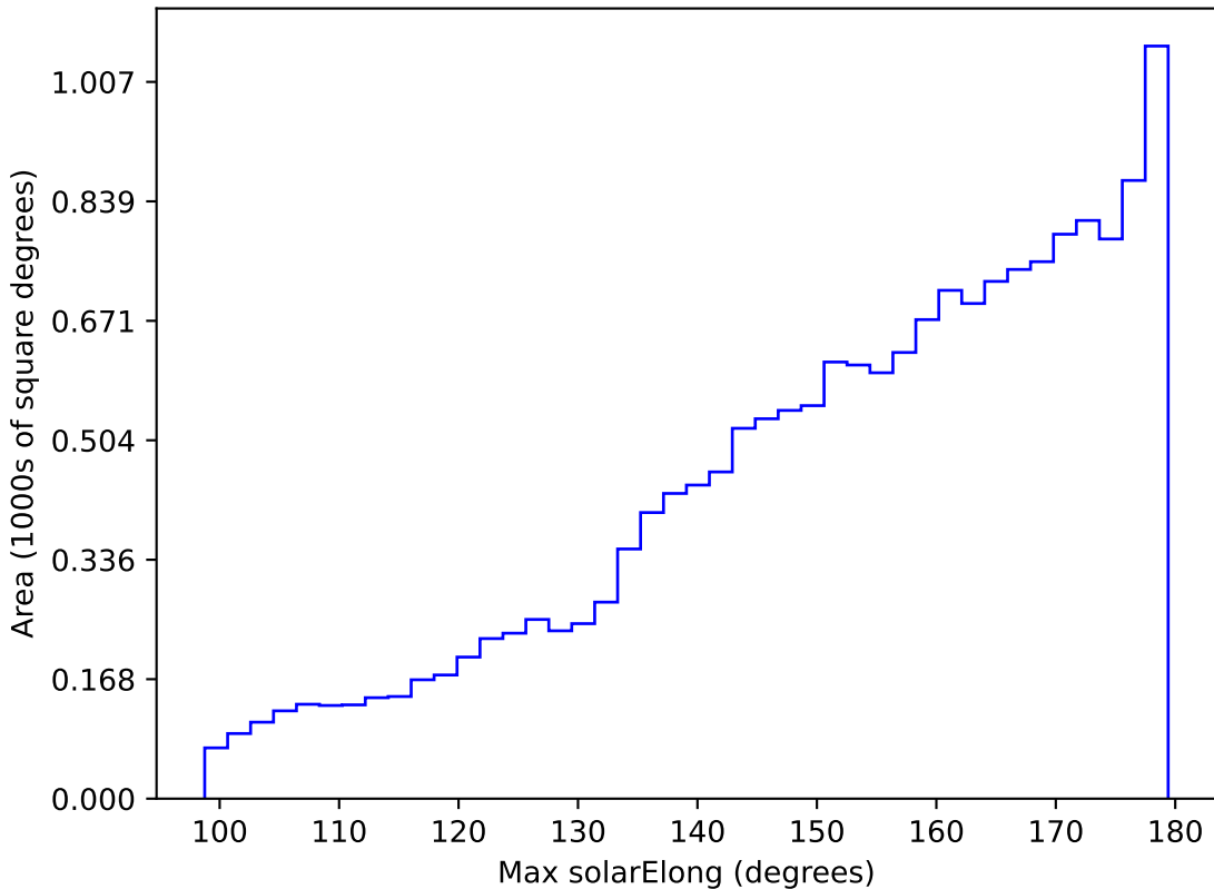
ddf_acor_sf20_lsf0_lsr0_v3.4_10yrs WFD r band: Max solarElong
