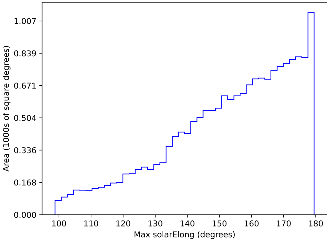
ddf_acor_sf20_lsf0_lsr0_v3.4_10yrs WFD i band: Max solarElong
