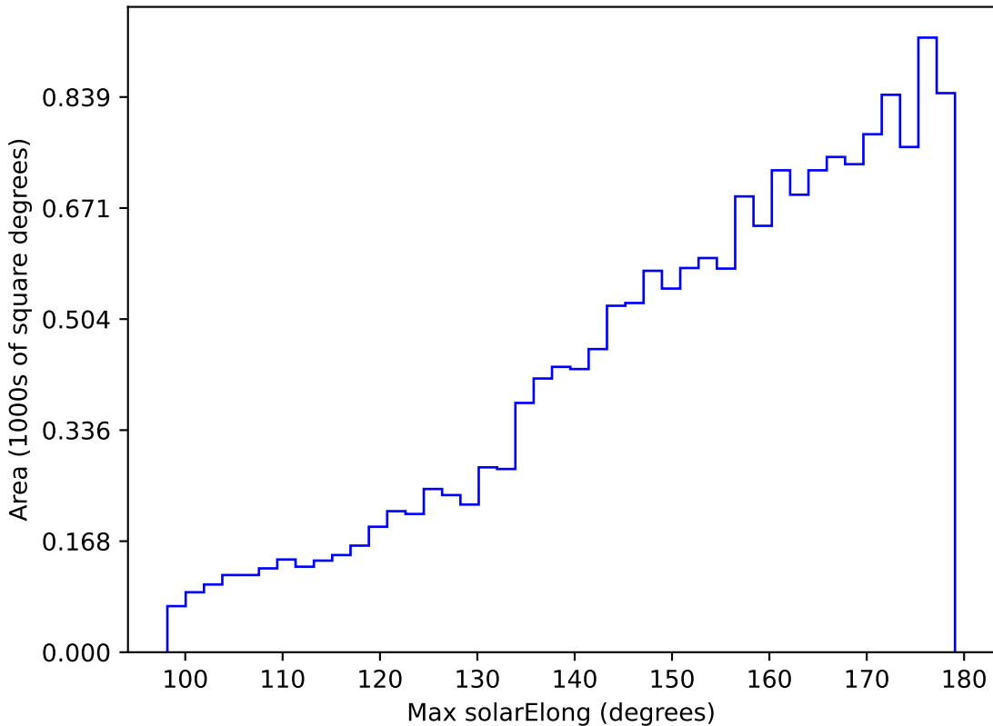
ddf_acor_sf20_lsf0_lsr0_v3.4_10yrs WFD g band: Max solarElong
