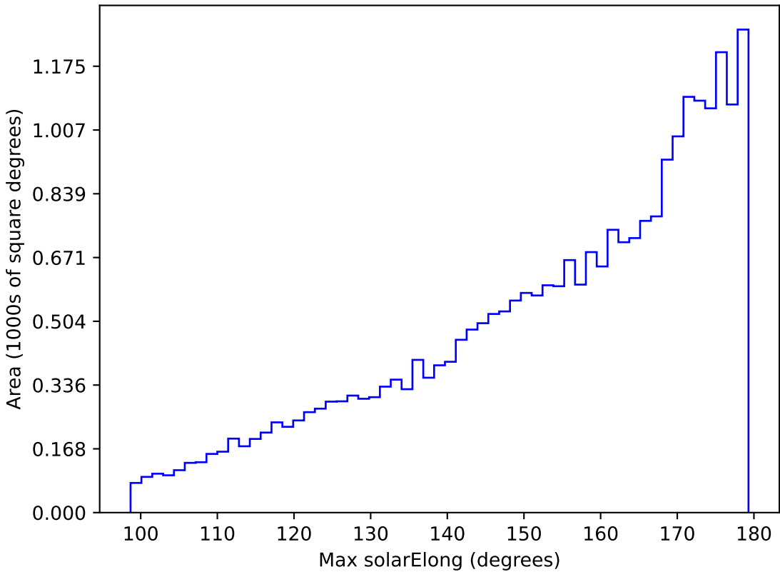
ddf_acor_sf20_lsf0_lsr0_v3.4_10yrs All sky z band: Max solarElong
