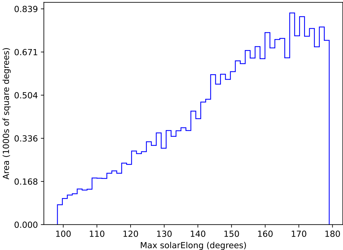
ddf_acor_sf20_lsf0_lsr0_v3.4_10yrs All sky u band: Max solarElong
