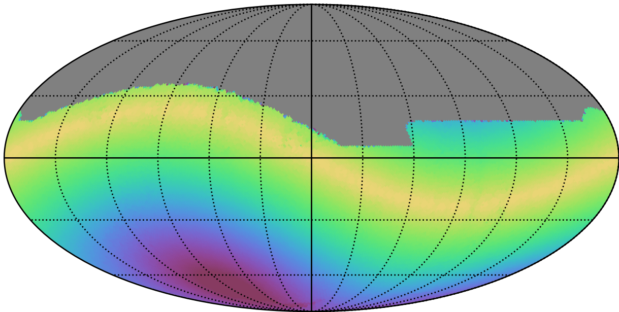
ddf_acor_sf20_lsf0_lsr0_v3.4_10yrs All sky r band: Max solarElong
