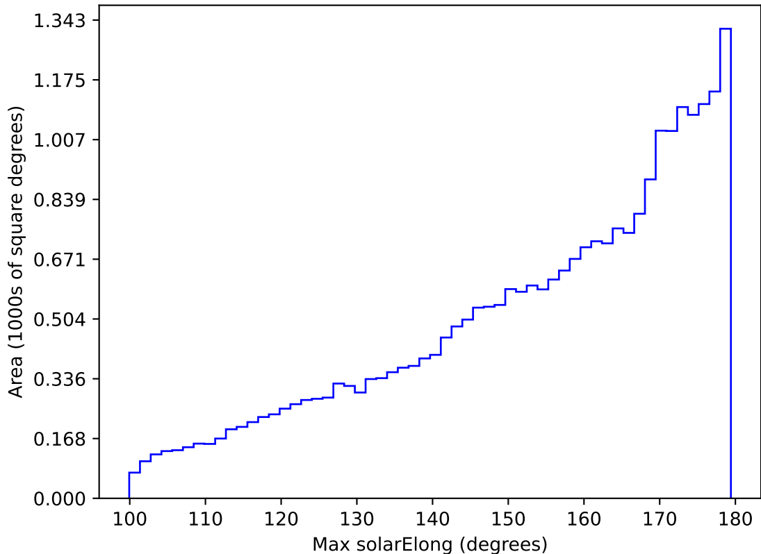
ddf_acor_sf20_lsf0_lsr0_v3.4_10yrs All sky r band: Max solarElong
