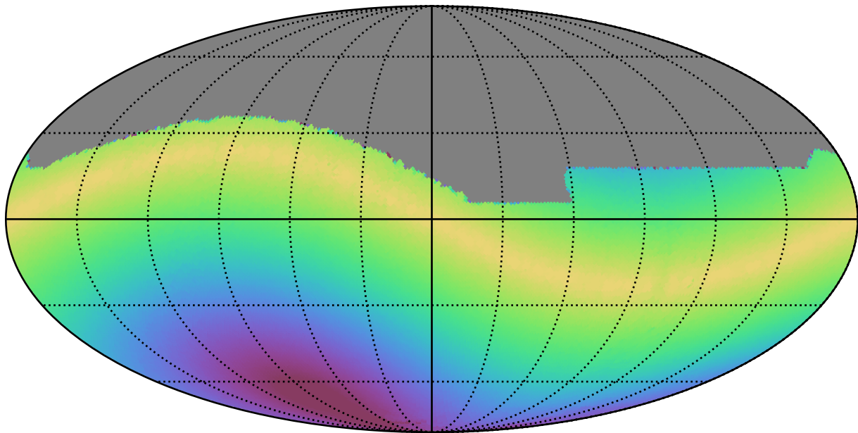
ddf_acor_sf20_lsf0_lsr0_v3.4_10yrs All sky i band: Max solarElong
