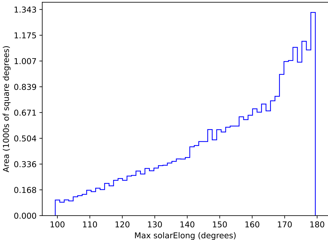
ddf_acor_sf20_lsf0_lsr0_v3.4_10yrs All sky i band: Max solarElong
