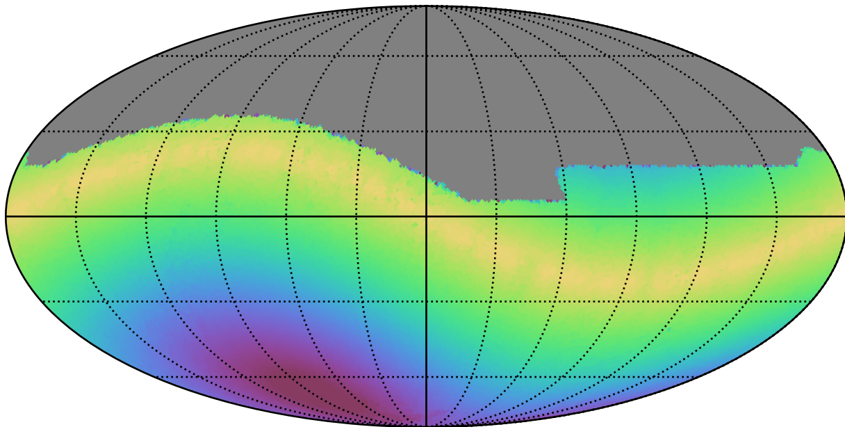
ddf_acor_sf20_lsf0_lsr0_v3.4_10yrs All sky g band: Max solarElong
