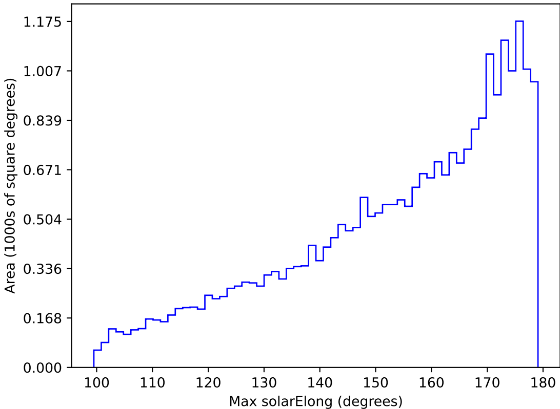
ddf_acor_sf20_lsf0_lsr0_v3.4_10yrs All sky g band: Max solarElong
