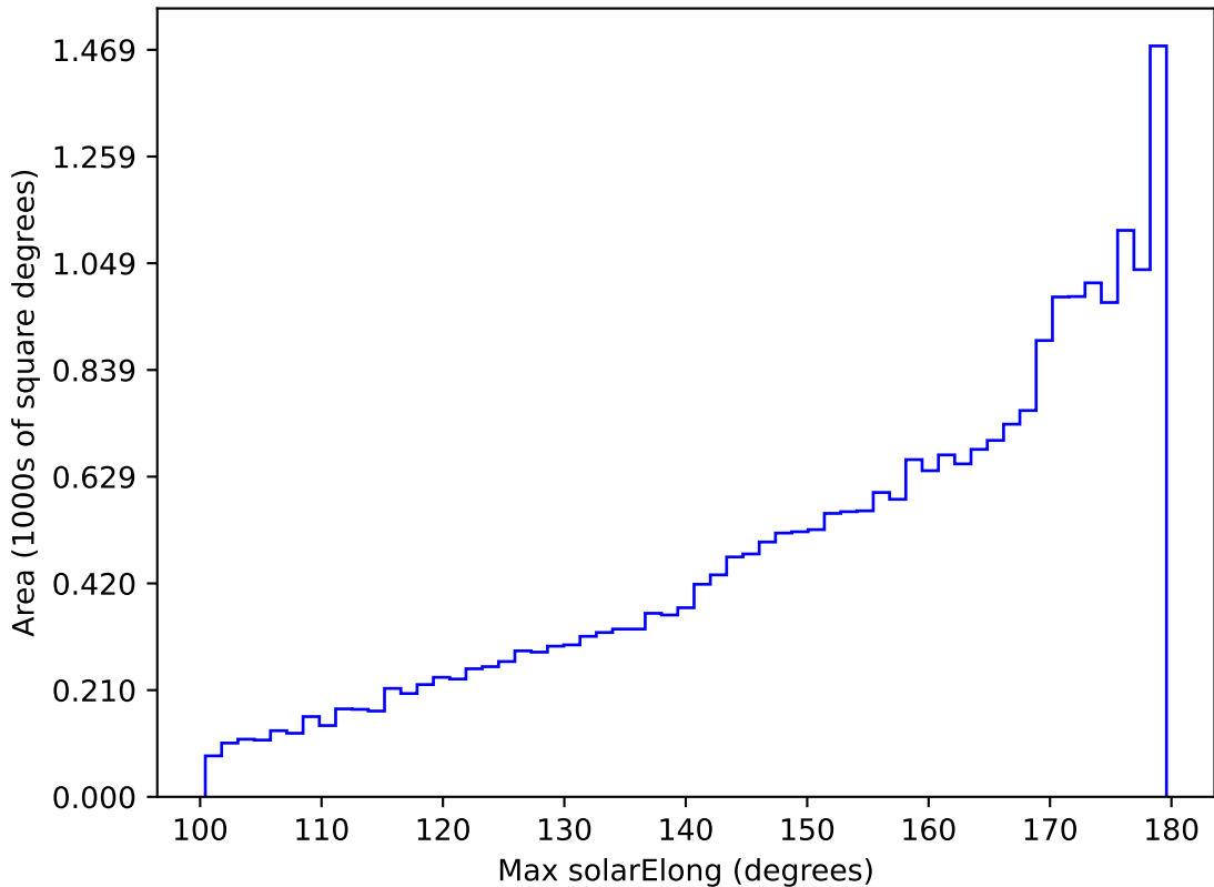
ddf_acor_sf20_lsf0_lsr0_v3.4_10yrs All sky all bands: Max solarElong
