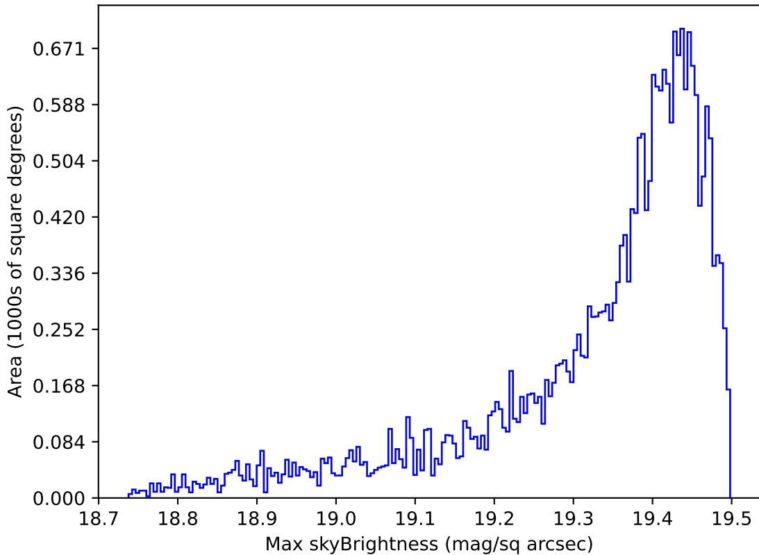
ddf_acor_sf20_lsf0_lsr0_v3.4_10yrs Yr 1 z band: Max skyBrightness
