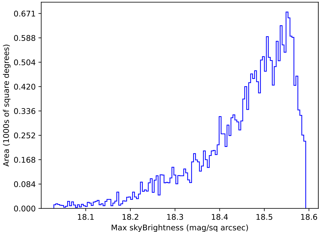
ddf_acor_sf20_lsf0_lsr0_v3.4_10yrs Yr 1 y band: Max skyBrightness
